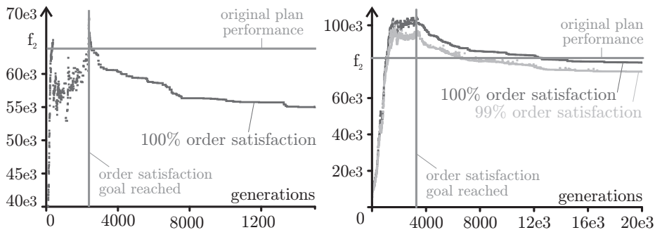
Fig. 3.1: For 642 orders (14% better).
