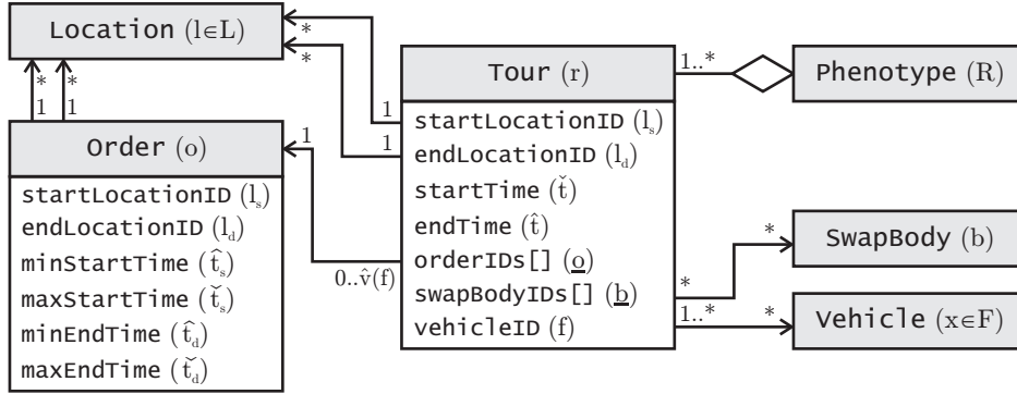
Fig. 1: The structure of the phenotypes R .
