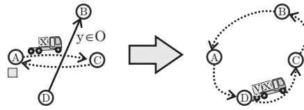
Fig. 2.2: Append an order.
