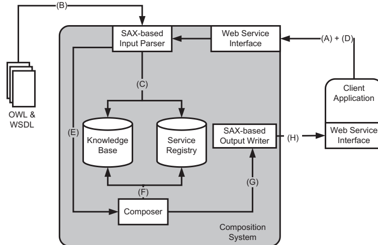
Figure 3: Example Composition System Implementation.
